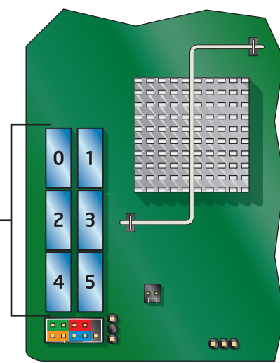
SATA Connector Detail
